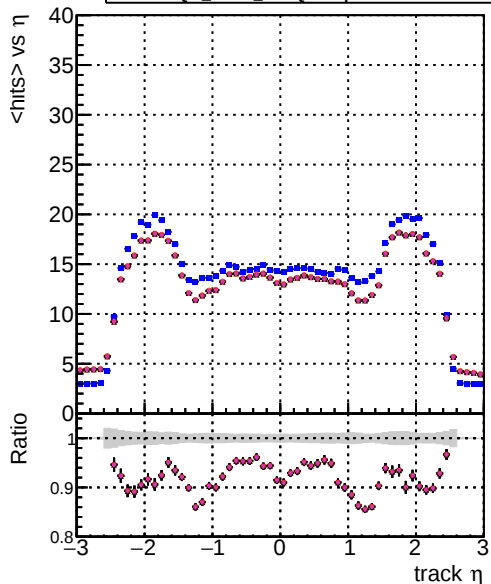
mean hit DOM CKE SortOCB DOM mkFit SortOCB-updated DOM mkFit SortOCB-updated newPLDNN DOM mkFit SortOCB-updated T1barDNN25
