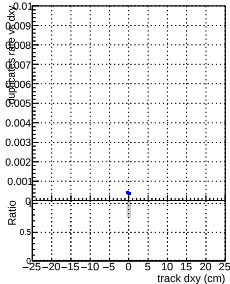
ewPLDNN thatBNN25
