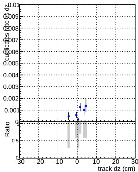
ewPLDNN thatBNN25
