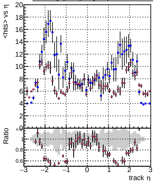
mean hits vs \eta DOM CKE SoftOCD DOM mkFit SoftOCD-updated DOM mkFit SoftOCD-updated-newPLDNN DOM mkFit SoftOCD-updated-TTbarDNN25
