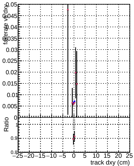
DOM GKE softGPD DOM GKE softGPD-updated DOM GKE softGPD-updated-TTbarNN25 DOM GKE softGPD-updated-TTbarNN25
