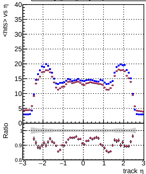
mean hit DOM_CKE_SortOCB DOM_mkFit_SortOCB-updated-newPLDNN DOM_mkFit_SortOCB-updated-TTbarDNN25
