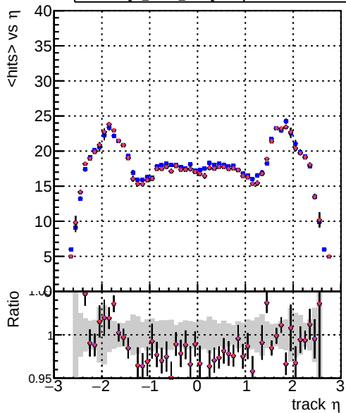
mean hit DOM_CKE_SortOCB DOM_mkFit_SortOCB-updated DOM_mkFit_SortOCB-updated-newPLDNN DOM_mkFit_SortOCB-updated-TTbarDNN25 DOM_mkFit_SortOCB-updated-TTbarDNN
