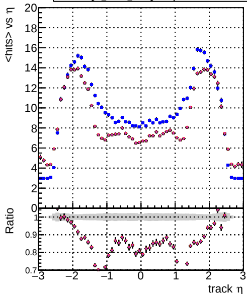
mean hits DOM CKE SortOCB DOM mkFit SortOCB-updated DOM mkFit SortOCB-updated-newPLDNN DOM mkFit SortOCB-updated-TTbarDNN25
