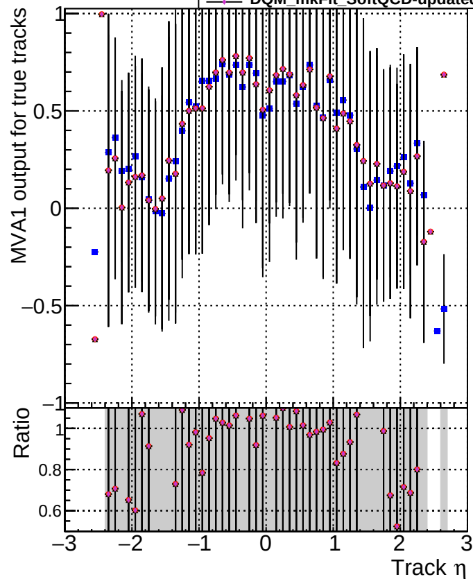
MVA1 of associated tracks (recoToSim) vs. track \eta Legend: DOM CKF softOCD DOM mkFit SoftOCD-updated DOM mkFit SoftOCD-updated-newPLDNN DOM mkFit SoftOCD-updated-TTbarDNN DOM mkFit SoftOCD-updated-TTbarDNN25
