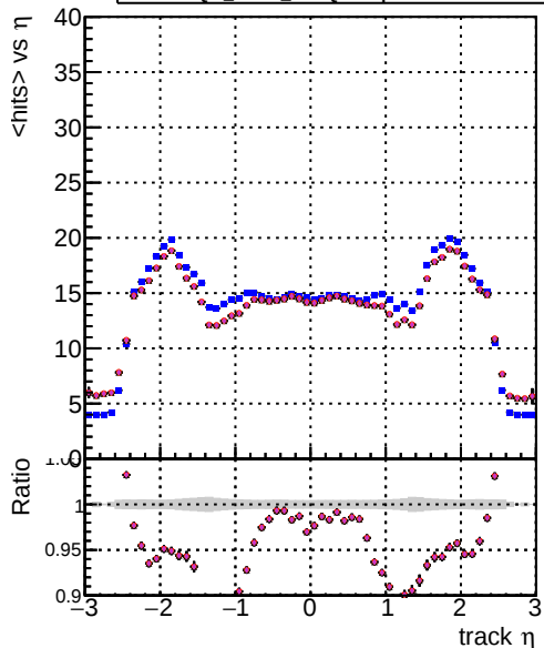
mean hits DOM CKE SortOCB DOM mkFit SortOCB-updated newPLDNN DOM mkFit SortOCB-updated TTbarDNN25 DOM mkFit SortOCB-updated TTbarDNN
