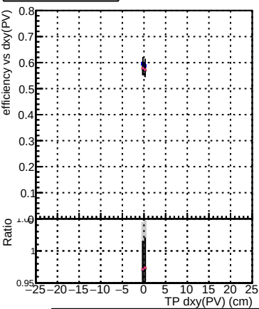
Efficiency vs Dxy(PV) Legend: DOM_CKF_SoftQCD DOM_mkFit_SoftQCD-updated DOM_mkFit_SoftQCD-updated-newPLDNN DOM_mkFit_SoftQCD-updated-TTbarDNN DOM_mkFit_SoftQCD-updated-TTbarDNN25
