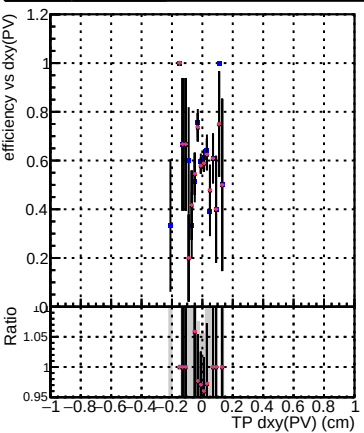
Efficiency vs Dxy(PV) Legend: DOM_CKF_SoftQCD DOM_mkFit_SoftQCD-updated DOM_mkFit_SoftQCD-updated-newPLDNN DOM_mkFit_SoftQCD-updated-TTbarDNN DOM_mkFit_SoftQCD-updated-TTbarDNN25
