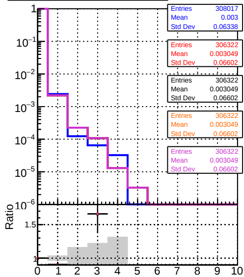
DOM_CKE_SortOCB DOM_mkFit_SortOCB-updated DOM_mkFit_SortOCB-updated-newPLDNN DOM_mkFit_SortOCB-updated-TTbarDNN DOM_mkFit_SortOCB-updated-TTbarDNN25 mean hit
