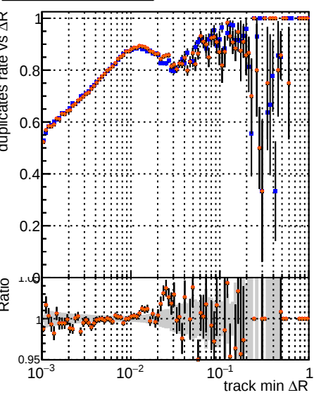
Legend: DOM, CKE, SoftQCD, DNN, DNN-updated, DNN-new, DNN-TTbar, DNN-DNN
