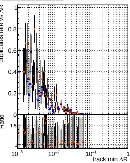
Fake rate vs ΔR(track, jet) Duplicates Rate vs ΔR(track, jet) Pileup rate vs ΔR(track, jet) Legend: DOM, CKE, SoftQCD, DNN, mkrfit, SoftQCD-updated, TtbarDNN
