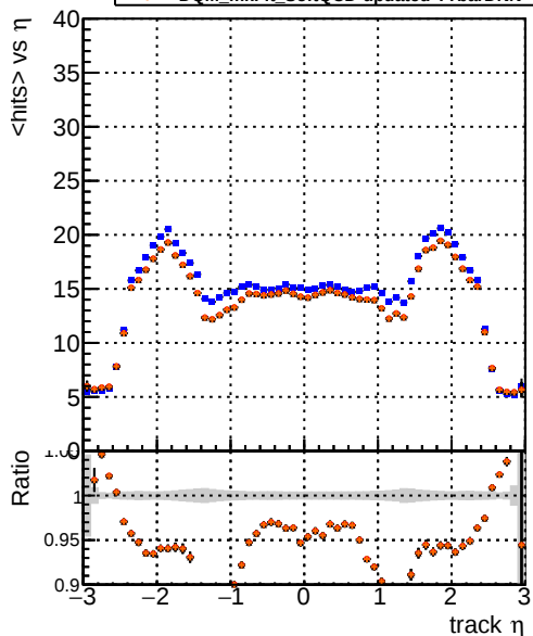
Legend: DOM_CKF_SoftQCD DOM_mkFit_SoftQCD-updated DOM_mkFit_SoftQCD-updated-newPLDNN DOM_mkFit_SoftQCD-updated-TTbarDNN mean hits
