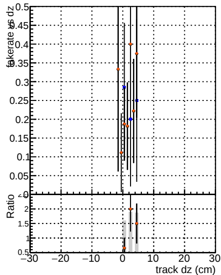
Fake rate vs dz DOM GKE softQCD DOM GKE softQCD-updated-new DOM GKE softQCD-updated-new+DNN
