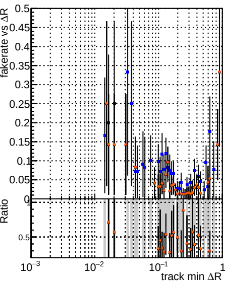
Fake rate vs \Delta R(\text{track}, \text{jet}) DOM CKE SoftQCD DOM mktFit SoftQCD-updated DOM mktFit SoftQCD-updated-TTbarDNN
