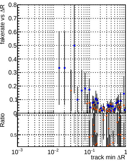
Fake rate vs ΔR(track, jet) Legend: DOM CKE SoftQCD SoftQCD-updated TtbarDNN
