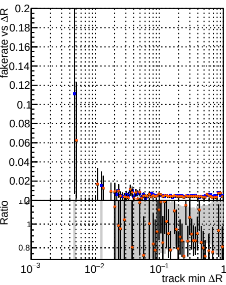
Fake rate vs \Delta R(\text{track, jet}) Legend: DOM CKE SoftQCD SoftQCD-updated mkFit mkFit-updated newPLDNN TTbarDNN
