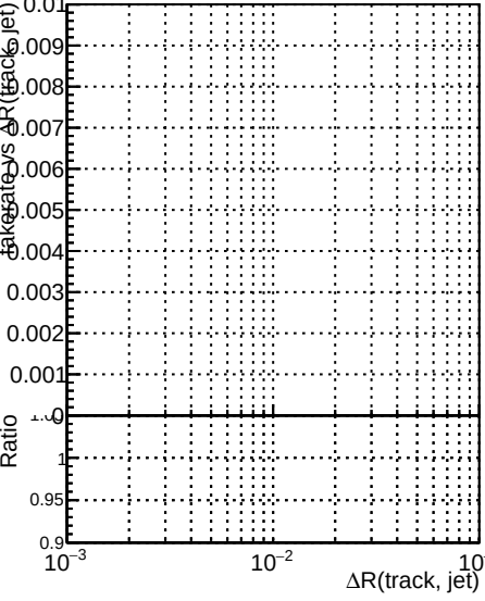
Fake rate vs \Delta R(\text{track, jet}) Legend: DOM, CKE, softQCD, DNN, mktfit, softQCD-updated, DNN-updated, T1barDNN
