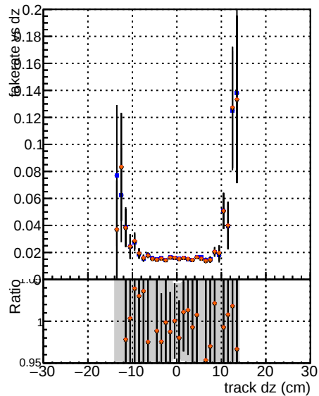
Fake rate vs dz —●— DOM GKE softQSP —●— DOM GKE softQSP updated-new PLDNN —●— DOM GKE softQSP updated-new PLDNN
