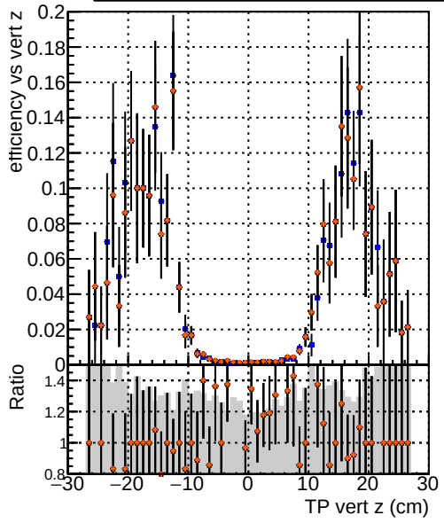
Efficiency vs vert z DOM_CKF_SoftQCD DOM_mkFit_SoftQCD-updated DOM_mkFit_SoftQCD-updated-newPLDNN DOM_mkFit_SoftQCD-updated-TTbarDNN
