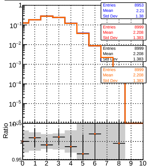
mean hit Legend: DQM_CKF_SoftQCD (blue line with circles) DQM_mkFit_SoftQCD-updated (red line with circles) DQM_mkFit_SoftQCD-updated-TPPLDNN (black line with circles) DQM_mkFit_SoftQCD-updated-TTbarDNN (orange line with circles)
