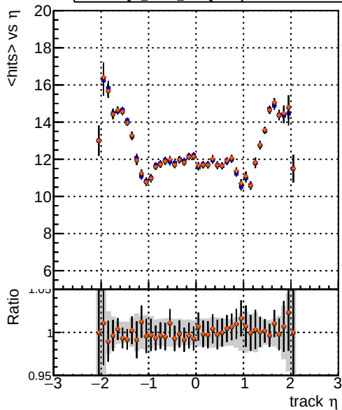
mean hit Legend: DQM_CKF_SoftQCD (blue line with circles) DQM_mkFit_SoftQCD-updated (red line with circles) DQM_mkFit_SoftQCD-updated-TPPLDNN (black line with circles) DQM_mkFit_SoftQCD-updated-TTbarDNN (orange line with circles)
