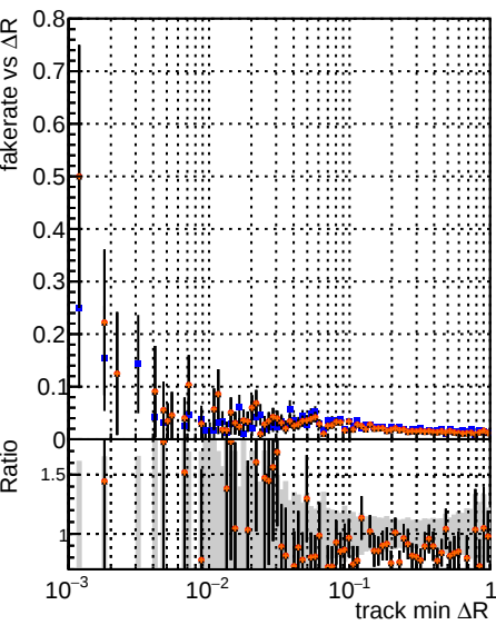
Fake rate vs ΔR(track, jet) Legend: DOM, CKE, SoftQCD, DNN, mktfit, SoftQCD-updated, TtbarDNN
