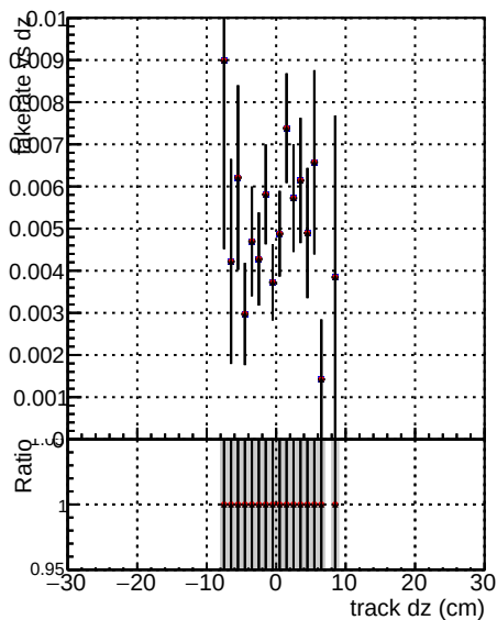
Fake rate vs dz DOM mkFit SoftQCD-updated DOM mkFit SoftQCD-updated-newPLDNN
