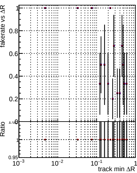
Legend: DQM_mkFit_SoftQCD-updated (grey), DQM_mkFit_SoftQCD-updated-newPLDNN (red), DQM_mkFit_SoftQCD-updated-TTbarDNN (black)
