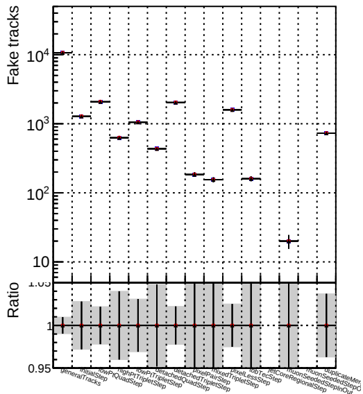
Number of tracks vs collection Legend: DQM_mkFit_SoftQCD-updated DQM_mkFit_SoftQCD-updated-newPLDNN DQM_mkFit_SoftQCD-updated-TTbarDNN
