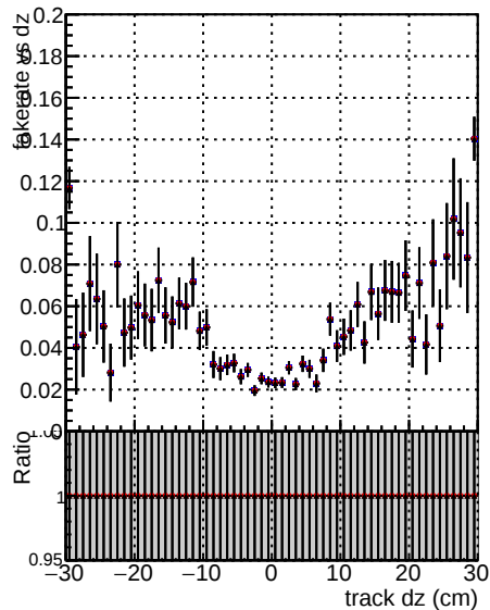
DOM mkFit SoftOCB-updated DOM mkFit SoftOCB-updated-newPLDNN DOM mkFit SoftOCB-updated-17hardDNN
