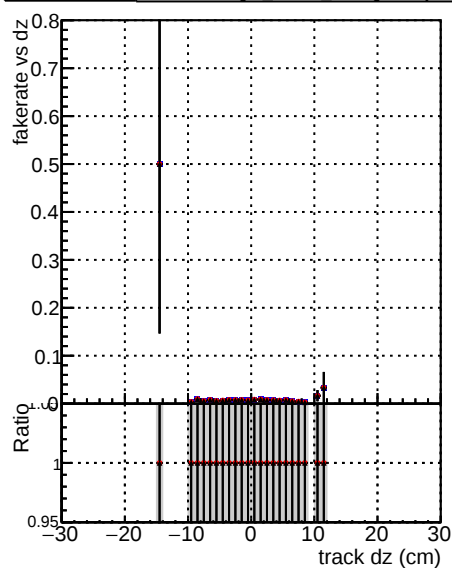
Fake rate vs dz Legend: DOM mkFit SoftQCD-updated newPLDNN DOM mkFit SoftQCD-updated HardDNN
