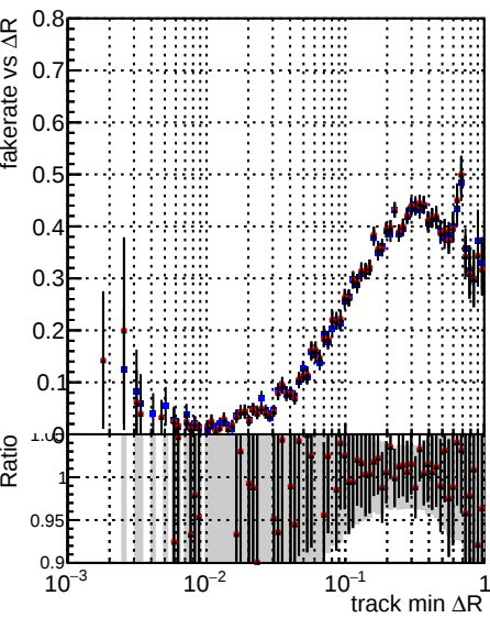
Legend: DQM_CKF_softQCD (blue circles), DQM_mkFit_SoftQCD-updated (red circles), DQM_mkFit_SoftQCD-updated-newPLDNN (black circles)
