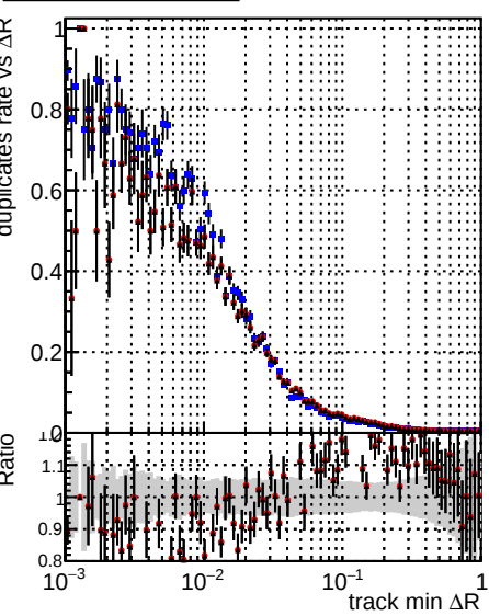
Legend: DQM_CKF_softQCD (blue squares), DQM_mkFit_SoftQCD-updated (red circles), DQM_mkFit_SoftQCD-updated-newPLDNN (black triangles)
