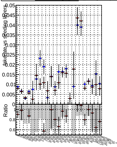
Fake rate vs. DOM CKF softOCB BQM-mkFit softOCB-updated BQM-mkFit softOCB-updated-newPLDNN
