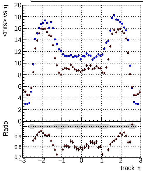
mean hits vs \eta Legend: DQM_CKF_softQCD (blue), DQM_mkFit_SoftQCD-updated (red), DQM_mkFit_SoftQCD-updated-newPLDNN (black)
