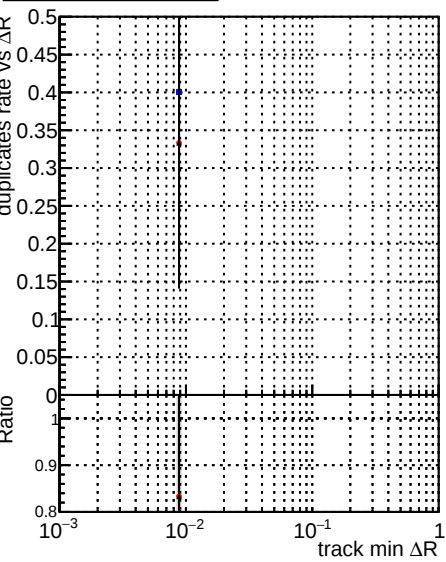
Legend: DQM_CKF_softQCD (blue squares), DQM_mkFit_SoftQCD-updated (red circles), DQM_mkFit_SoftQCD-updated-newPLDNN (black line)
