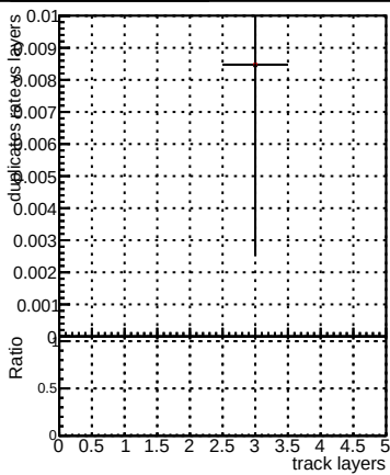
Legend: DQM_CKF_softQCD (blue dots), DQM_mkFit_SoftQCD-updated (red line), DQM_mkFit_SoftQCD-updated-newPLDNN (black line)
