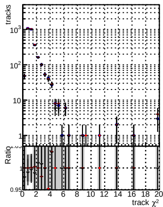
N of reco track vs. \chi^2 for DOM CKE T-base, DOM CKE T-retrainOldFiles113, and DOM CKE T-retrainOldFiles125 v2
