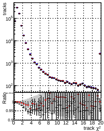
N of reco track vs. s DOM CKE TT retrainOldFiles 113 DOM CKE TT retrainOldFiles 125 v2
