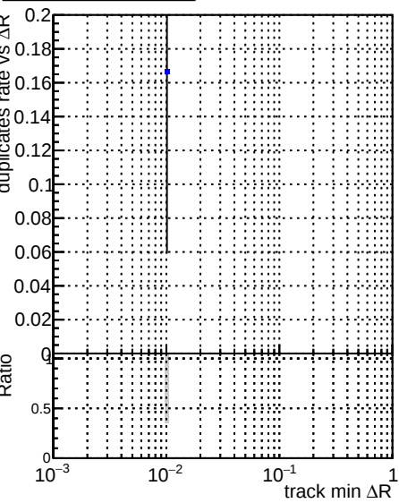
Legend: DQM_CKF_TTbase (blue dots), DQM_CKF_TT_retrainOldFiles113 (red dots), DQM_CKF_TT_retrainOldFiles125_v2 (black dots)
