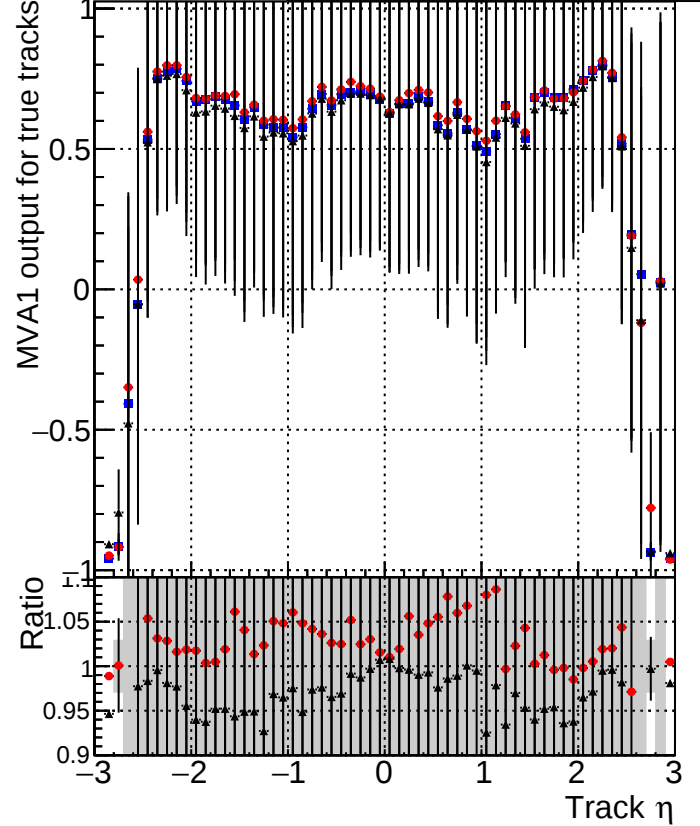
MVA1 of associated tracks (recoToSim) vs. track \eta Legend: DQM_CKF_TTbase (blue squares) DQM_CKF_TT_retrainOldFiles113 (red circles) DQM_CKF_TT_retrainOldFiles125_v2 (black triangles)
