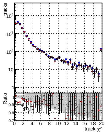
N of reco track vs. \chi^2 DOM CKF TTbase DOM CKF TT retrainOldFiles113 DOM CKF TT retrainOldFiles125 v2
