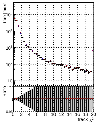
N of reco track vs. \chi^2 for retrain0113 noSel
