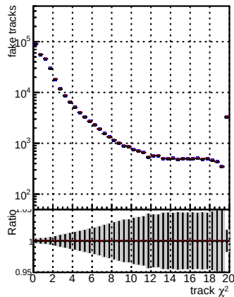
N of reco track vs. \chi^2 for retrain0113 V2 noSel
