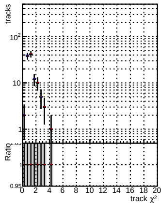
N of reco track vs. \chi^2 for Files113 noSel
