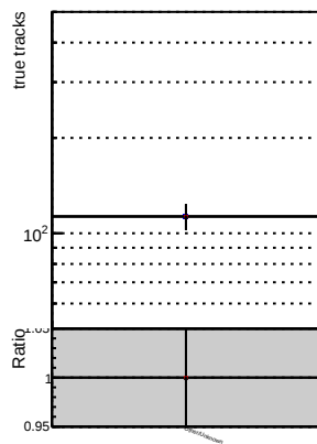
N of reco track vs. \chi^2 for Files113 noSel
