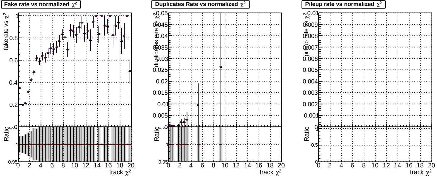
Fake rate vs. DOM CKF TT base noSel DOM CKF TT retrainOldFiles113 noSel DOM CKF TT retrainOldFiles125 v2 noSel
