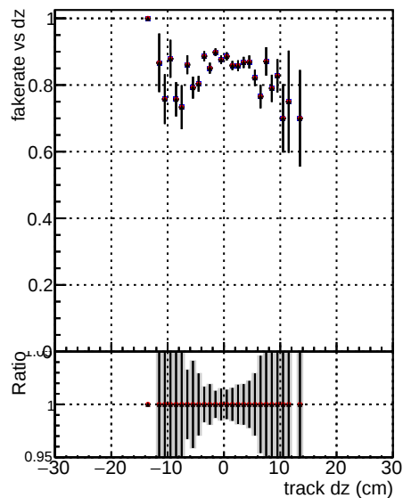
Fake rate vs dz Legend: DOM CKF TT base noSel DOM CKF TT retrainOldFiles113 noSel DOM CKF TT retrainOldFiles125 v2 noSel
