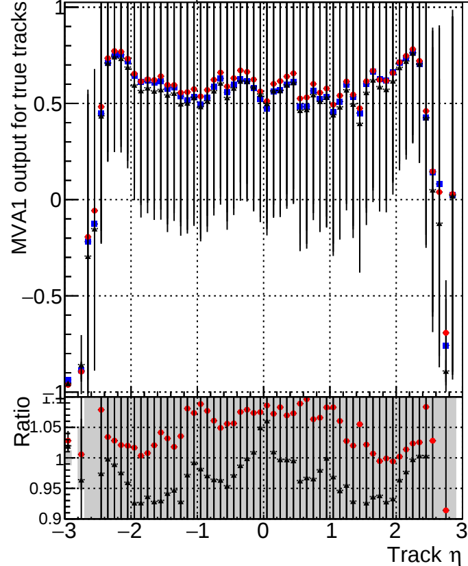
MVA1 of associated tracks (recoToSim) vs. track \eta Legend: DQM_CKF_TT_base_noSel (blue squares) DQM_CKF_TT_retrainOldFiles113_noSel (red circles) DQM_CKF_TT_retrainOldFiles125_v2_noSel (black stars)
