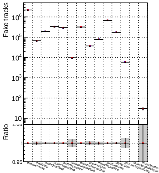
Number of tracks vs collection Legend: DQM_CKF_TT_base_noSel (Blue line with circles) DQM_CKF_TT_retrainOldFiles113_noSel (Red line with circles) DQM_CKF_TT_retrainOldFiles125_v2_noSel (Black line with circles)
