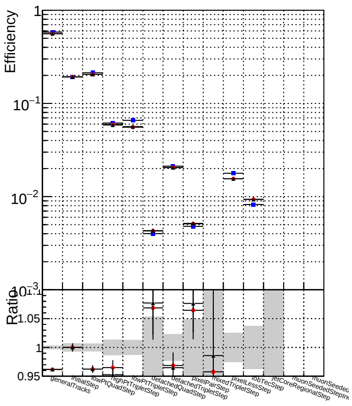
DQM_mkFit_TT_base_noSel DQM_mkFit_TT_base_8iter_noSel DQM_mkFit_TT_retrainOldFiles_v2_8iter2_noSel
