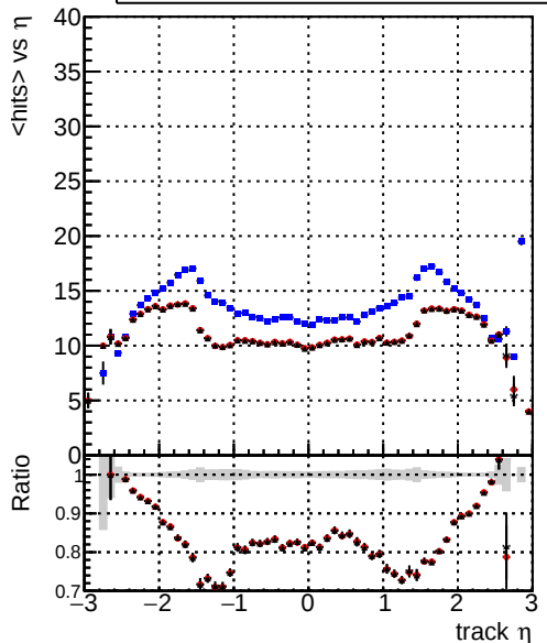
mean hit — DQM_mkFit_TT_base_noSel — DQM_mkFit_TT_base_8iter_noSel — DQM_mkFit_TT_retrainOldFiles_v2_8iter2_noSel
