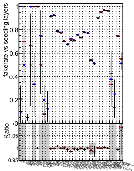
Fake rate vs. —■— DGM mkFit TT base noSel —●— DGM mkFit TT base 8iter noSel —▲— DGM mkFit TT retrainOldFiles v2 8iter2 noSel
