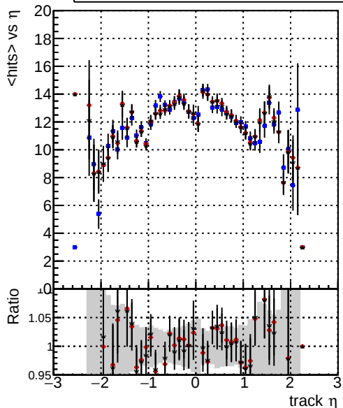
DQM_mkFit_TT_base_noSel DQM_mkFit_TT_base_8iter_noSel DQM_mkFit_TT_retrainOldFiles_v2_8iter2_noSel mean hit
