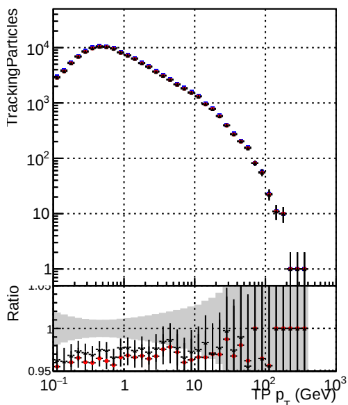
★ DQM_mkFit_TT_base_noSel ★ DQM_mkFit_TT_base_8iter_noSel ★ DQM_mkFit_TT_retrainOldFiles_v2_8iter2_noSel
